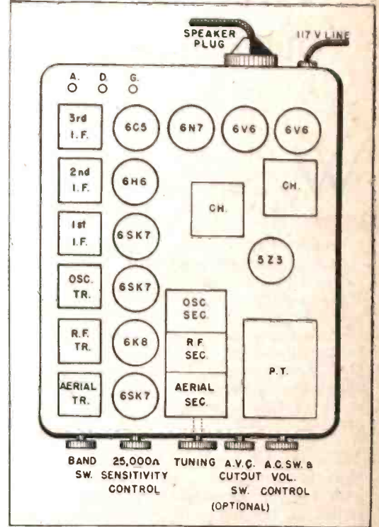
The complete diagram of Mr. Emmett's receiver is shown at top of page. Above is the chassis layout and below, the power pack.
