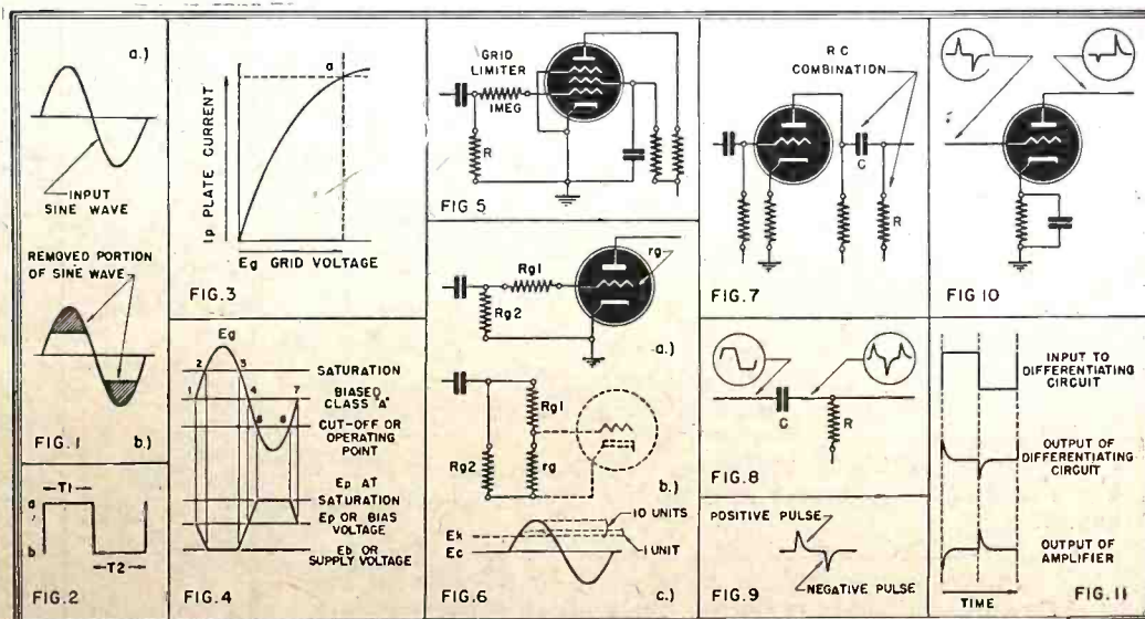
Fig. 1—Before and after clipping. Fig. 2—Ideal square wave. Fig. 3—Dynamic E_g-I_p curve. Fig. 4—Making a square wave. Fig. 5—Limiting resistor. Fig. 6—How it works. Fig. 7—Differentiator circuit. Fig. 8—Pulsing circuit. Fig. 9—Positive and negative pulses. Fig. 10—Positive pulse amplifier (negative clipped). Fig. 11—Pulse wave forms (not to scale).
