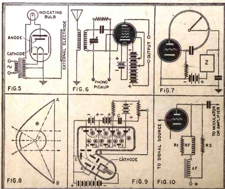
Fig. 5—An intrusion detector. Fig. 6—A space-charge circuit. Fig. 7—Ultra-high-frequency transceiver. Fig. 8—UHF reflector. Fig. 9—Bent electron multiplier. Fig. 10—A relaxation oscillator.
