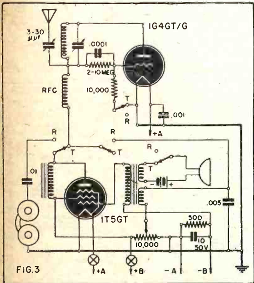
Complete circuit with switching arrangement.
