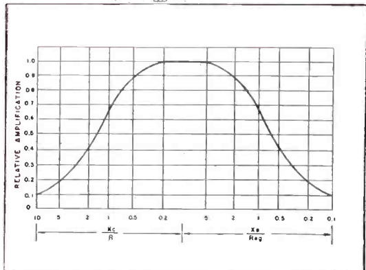
Fig. 1—The universal amplification curve.
