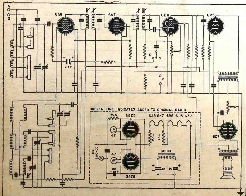
A converted RCA 85BK (85BT). The reader should compare this with the original schematic.
