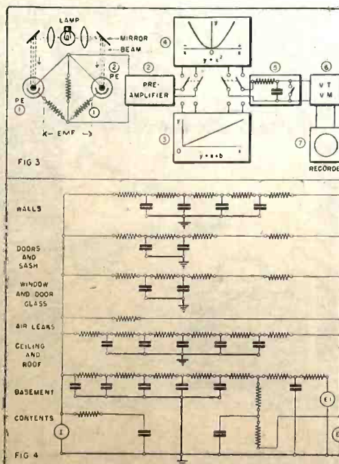
Fig. 3—"Glamour checker" for measuring silk stocking sheerness. Figs. 4 and 5—Thermal network of building and its control system.
