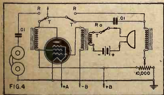
A simpler circuit using impedance coupling.
